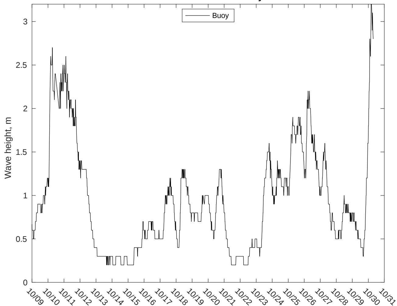
NDBC 42036 vs CMEMS Waves: 10 to 16 day forecast
