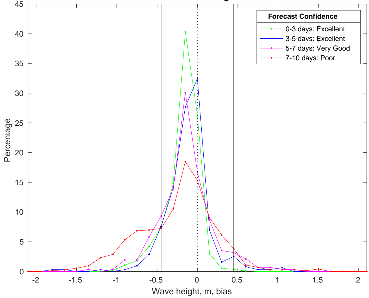
NDBC 42036 vs CMEMS Waves Bias Histogram: 30-Oct-2025
