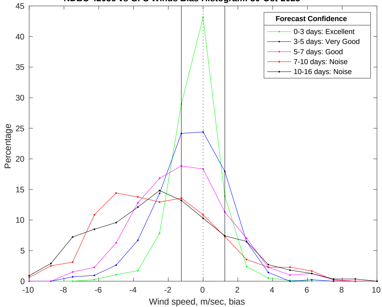
NDBC 42036 vs GFS Winds Bias Histogram: 30-Oct-2025
