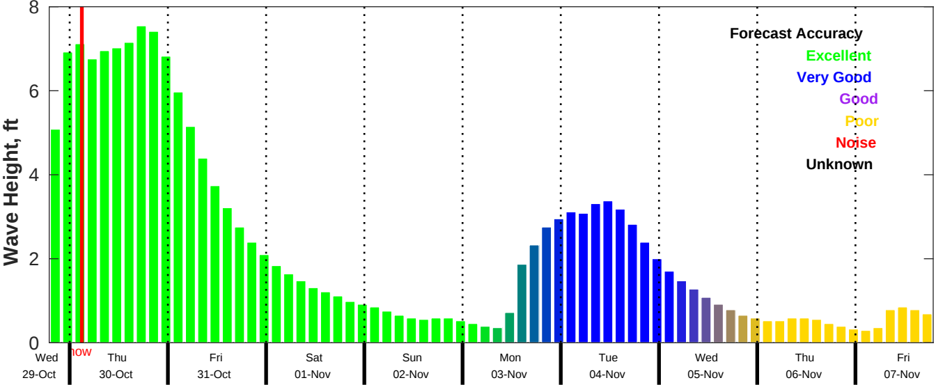
CMEMS Wave Forecast for NDBC 42036 from 29-Oct-2025 19:00:00 to 07-Nov-2025 19:00:00
