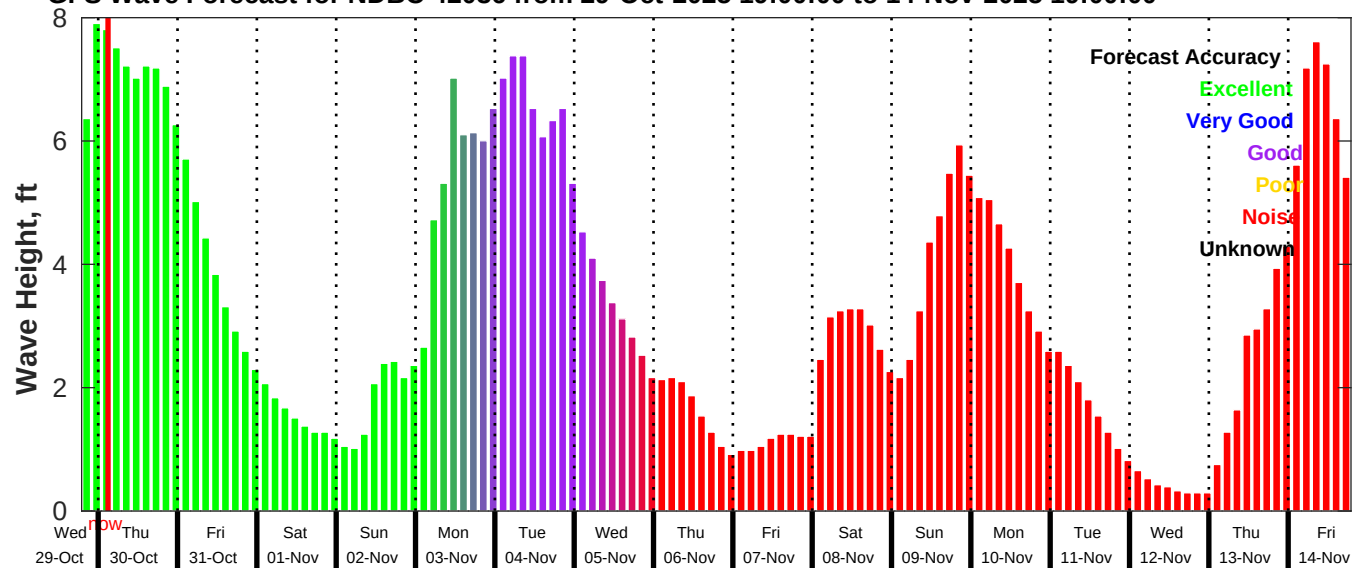
GFS Wave Forecast for NDBC 42036 from 29-Oct-2025 19:00:00 to 14-Nov-2025 19:00:00
