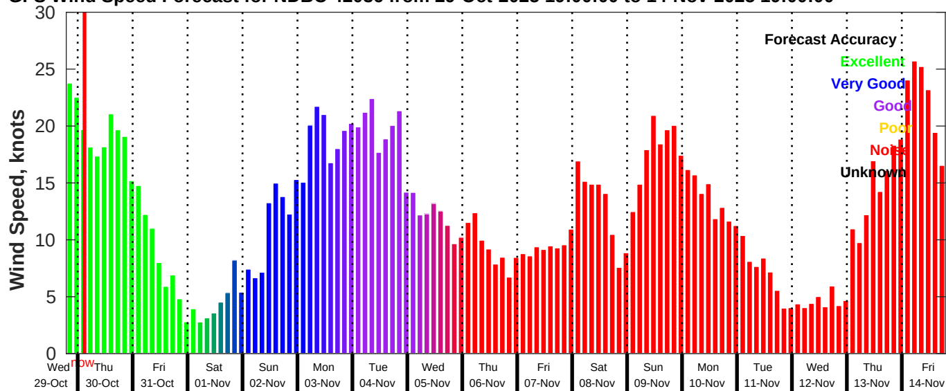
GFS Wind Speed Forecast for NDBC 42036 from 29-Oct-2025 19:00:00 to 14-Nov-2025 19:00:00
