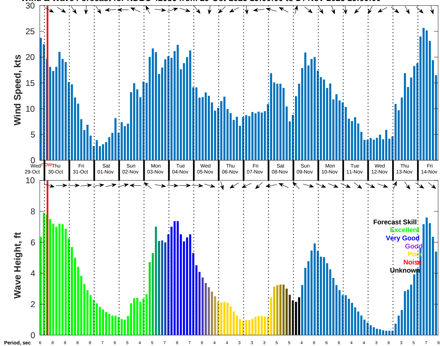
Wind & Wave Forecast for NDBC 42036 from 29-Oct-2025 19:00:00 to 14-Nov-2025 19:00:00
