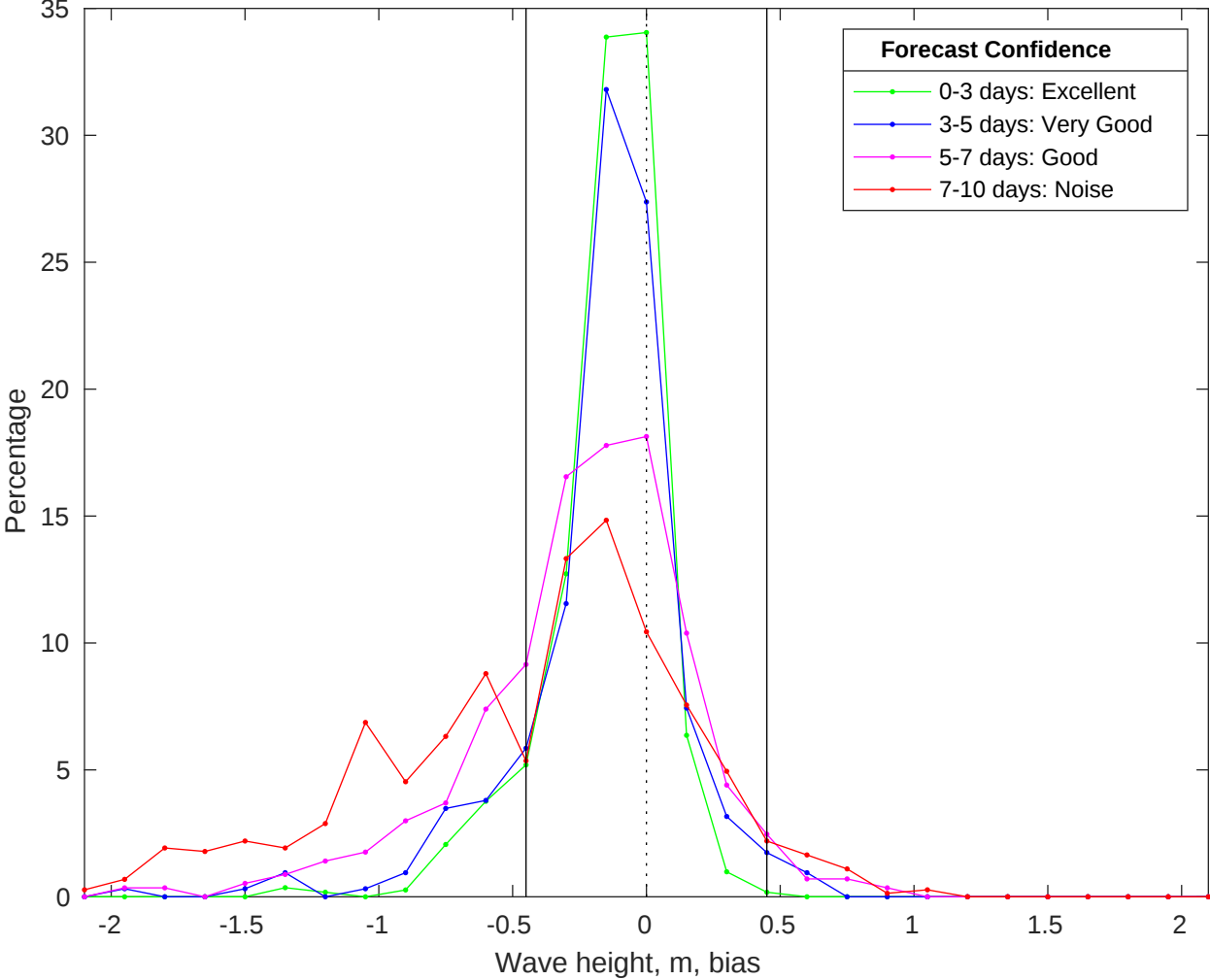
NDBC 42040 vs CMEMS Waves Bias Histogram: 30-Oct-2025
