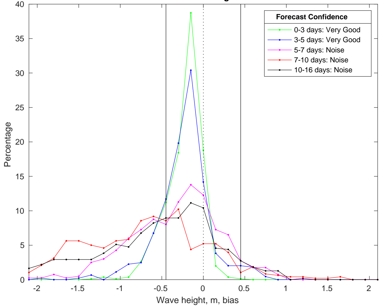
NDBC 42040 vs GFS Waves Bias Histogram: 30-Oct-2025
