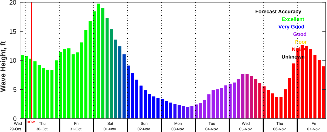
CMEMS Wave Forecast for NDBC 44008 from 29-Oct-2025 20:00:00 to 07-Nov-2025 20:00:00
