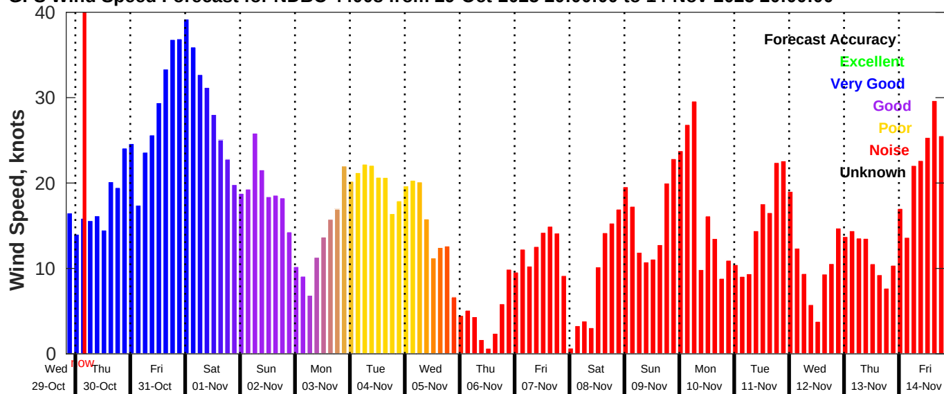
GFS Wind Speed Forecast for NDBC 44008 from 29-Oct-2025 20:00:00 to 14-Nov-2025 20:00:00
