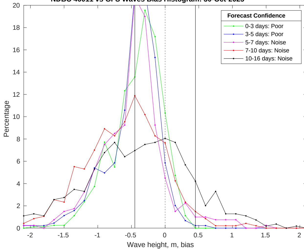
NDBC 46011 vs GFS Waves Bias Histogram: 30-Oct-2025
