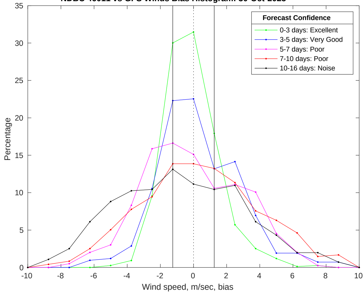
NDBC 46011 vs GFS Winds Bias Histogram: 30-Oct-2025
