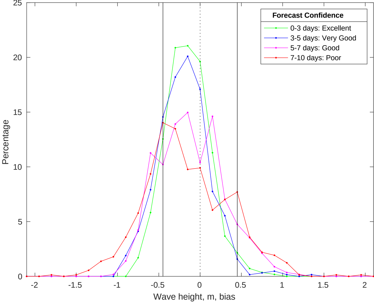
NDBC 46054 vs CMEMS Waves Bias Histogram: 30-Oct-2025
