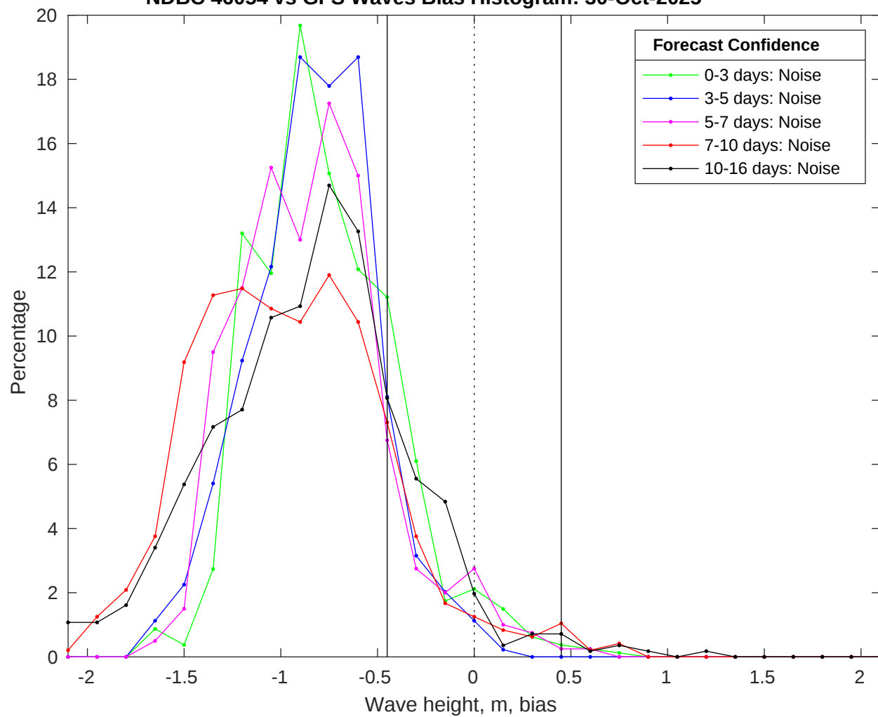
NDBC 46054 vs GFS Waves Bias Histogram: 30-Oct-2025
