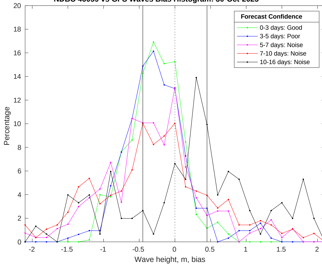
NDBC 46059 vs GFS Waves Bias Histogram: 30-Oct-2025
