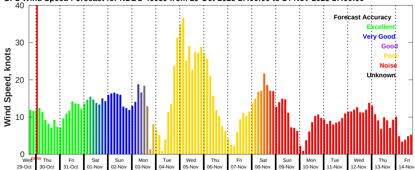
GFS Wind Speed Forecast for NDBC 46059 from 29-Oct-2025 17:00:00 to 14-Nov-2025 17:00:00
