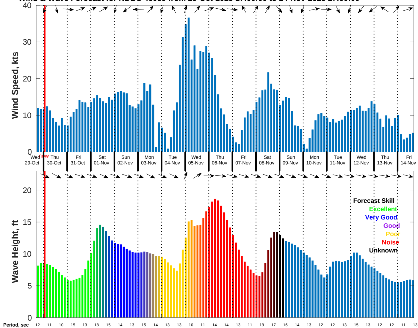
Wind & Wave Forecast for NDBC 46059 from 29-Oct-2025 17:00:00 to 14-Nov-2025 17:00:00
