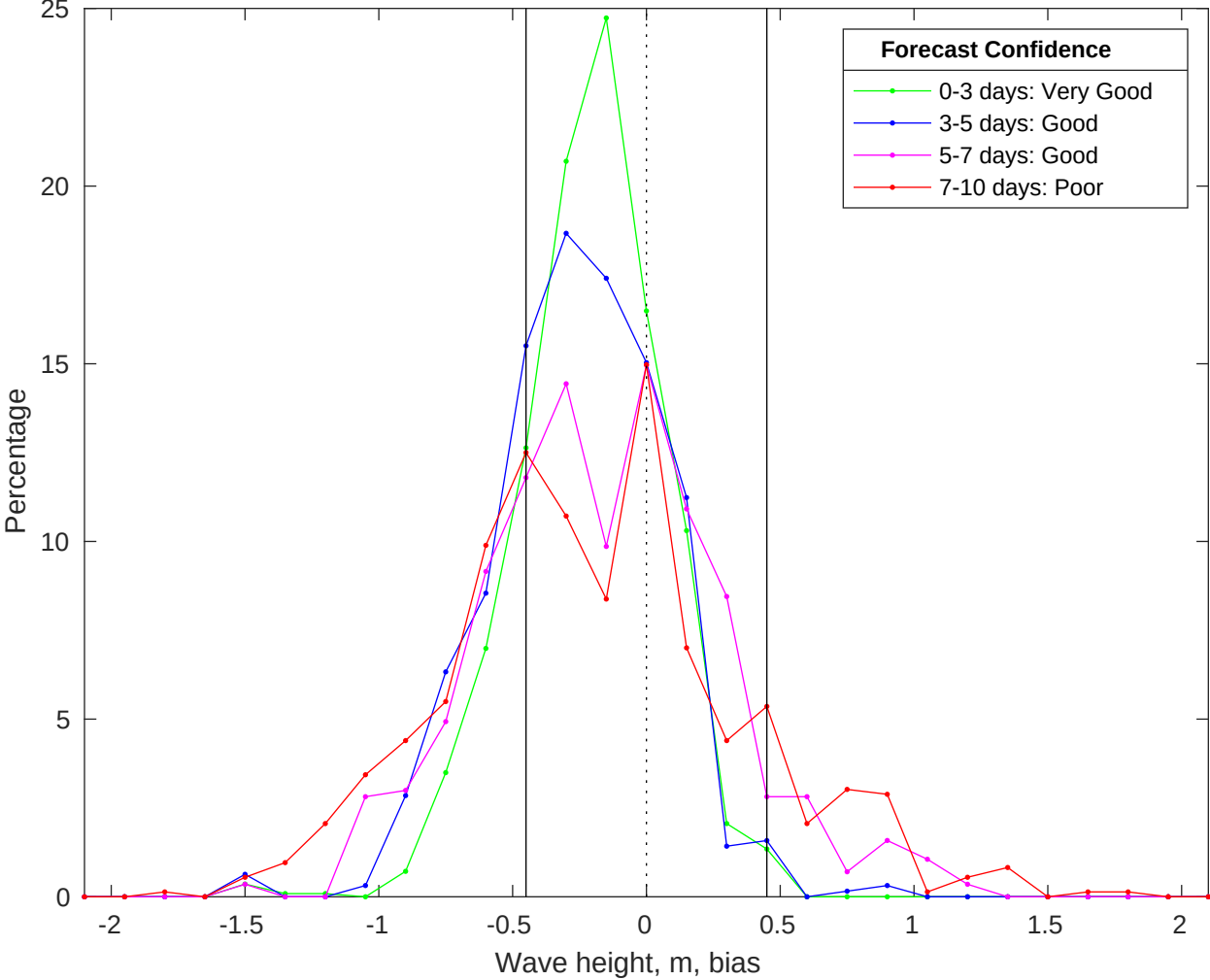
NDBC 46069 vs CMEMS Waves Bias Histogram: 30-Oct-2025
