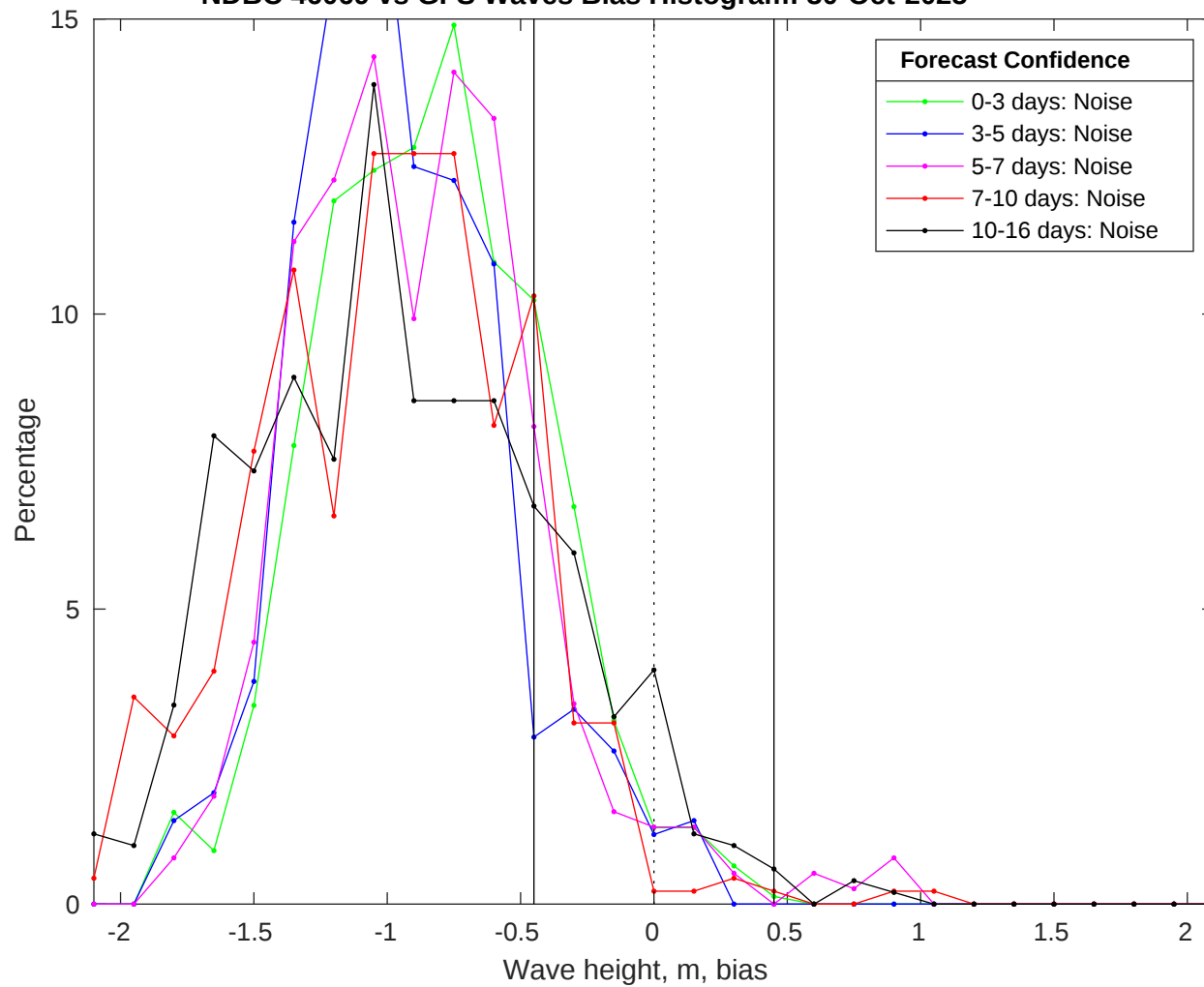
NDBC 46069 vs GFS Waves Bias Histogram: 30-Oct-2025
