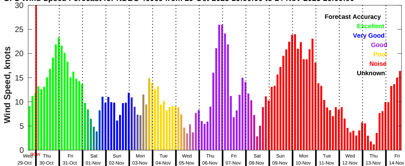
GFS Wind Speed Forecast for NDBC 46069 from 29-Oct-2025 16:00:00 to 14-Nov-2025 16:00:00
