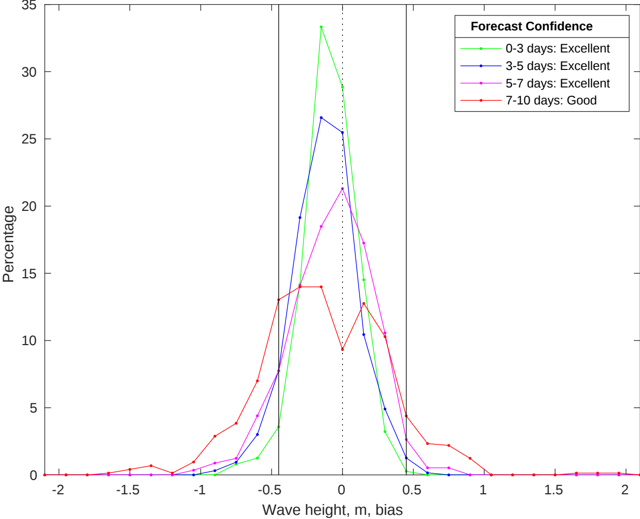
NDBC 46215 vs CMEMS Waves Bias Histogram: 30-Oct-2025
