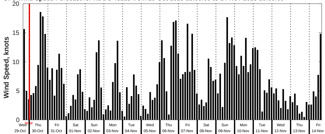
GFS Wind Speed Forecast for NDBC 46215 from 29-Oct-2025 16:00:00 to 14-Nov-2025 16:00:00
