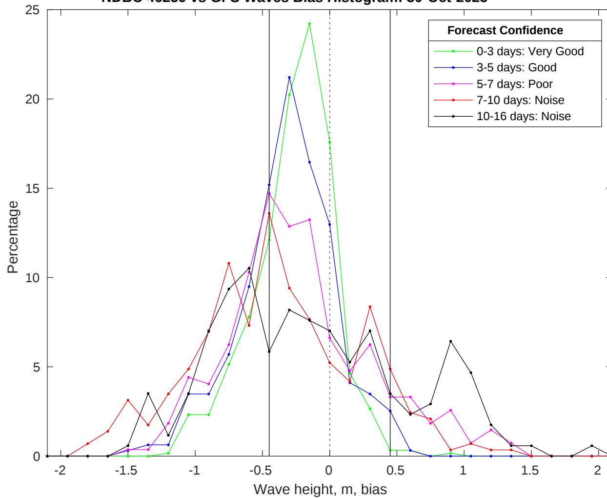
NDBC 46259 vs GFS Waves Bias Histogram: 30-Oct-2025
