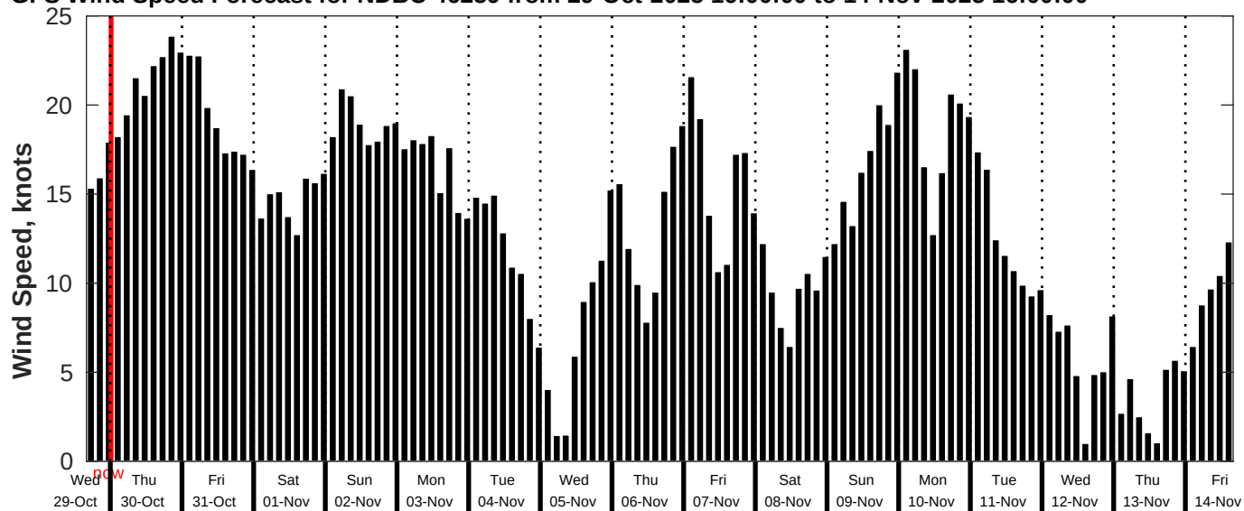
GFS Wind Speed Forecast for NDBC 46259 from 29-Oct-2025 16:00:00 to 14-Nov-2025 16:00:00
