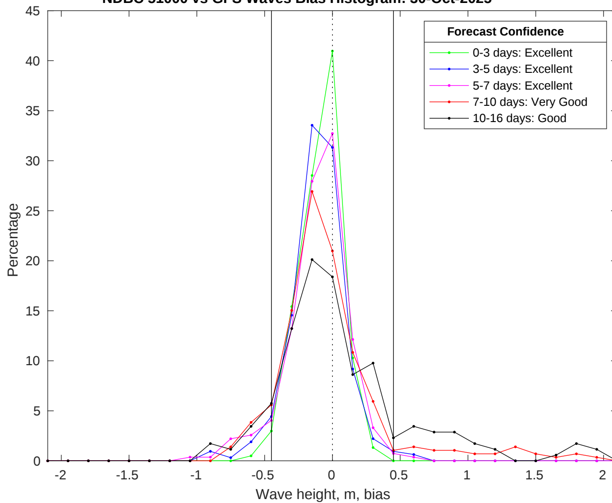
NDBC 51000 vs GFS Waves Bias Histogram: 30-Oct-2025
