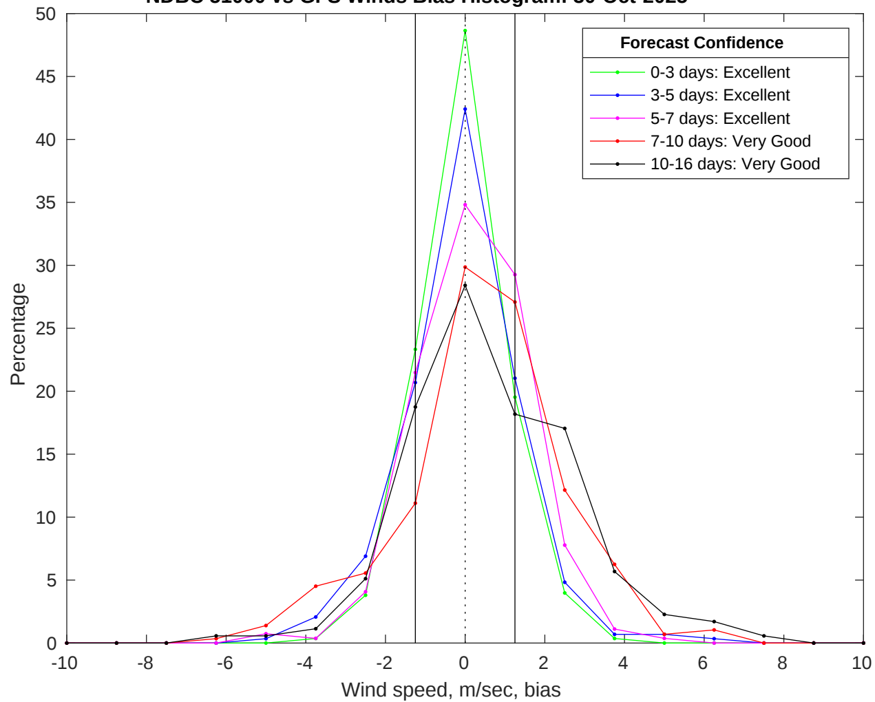
NDBC 51000 vs GFS Winds Bias Histogram: 30-Oct-2025
