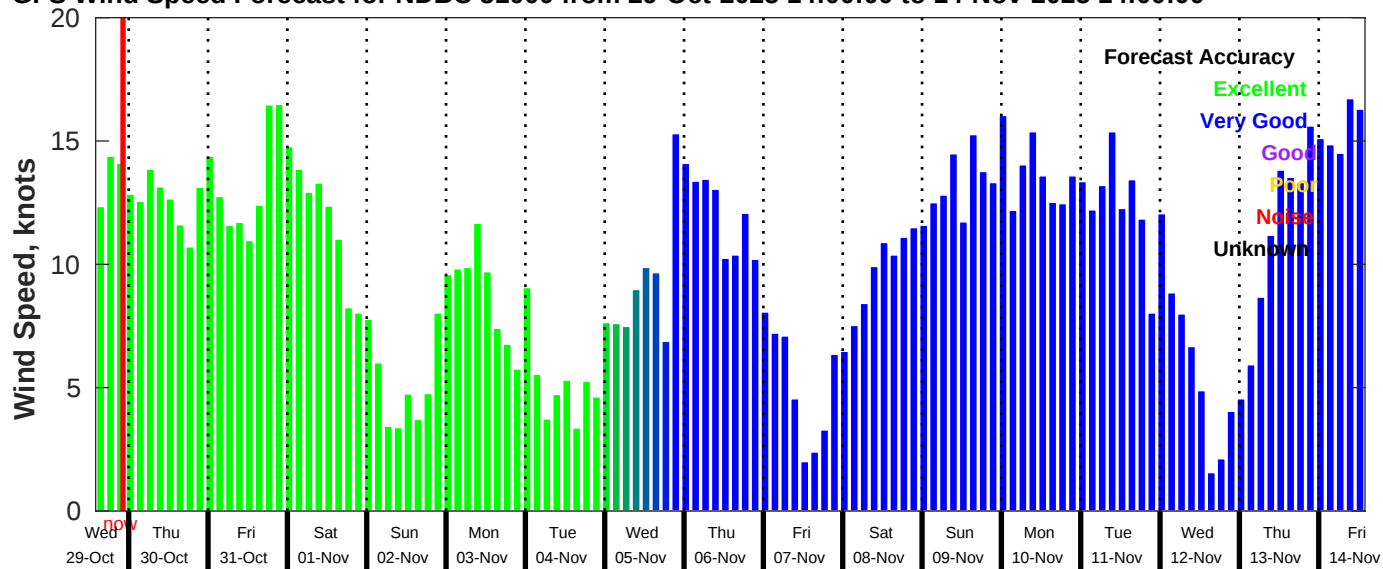
GFS Wind Speed Forecast for NDBC 51000 from 29-Oct-2025 14:00:00 to 14-Nov-2025 14:00:00
