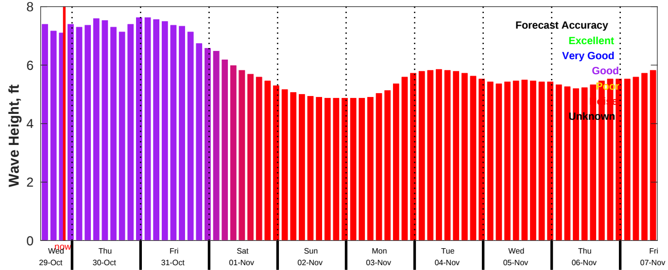
CMEMS Wave Forecast for NDBC 51209 from 29-Oct-2025 13:00:00 to 07-Nov-2025 13:00:00
