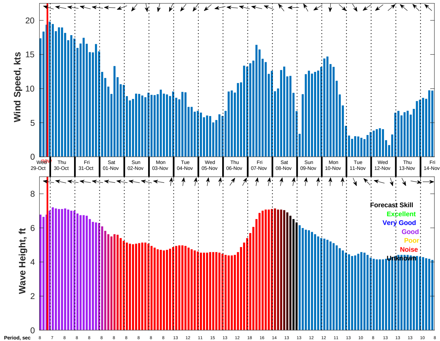
Wind & Wave Forecast for NDBC 51209 from 29-Oct-2025 13:00:00 to 14-Nov-2025 13:00:00
