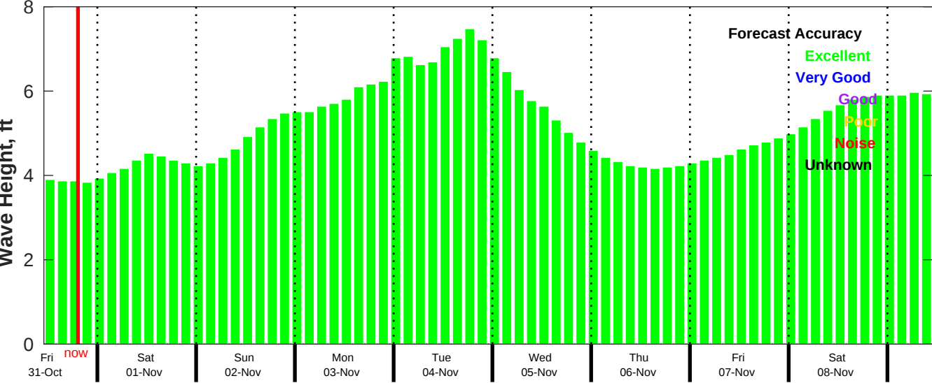
CMEMS Wave Forecast for NDBC 52211 from 30-Oct-2025 11:00:00 to 08-Nov-2025 11:00:00
