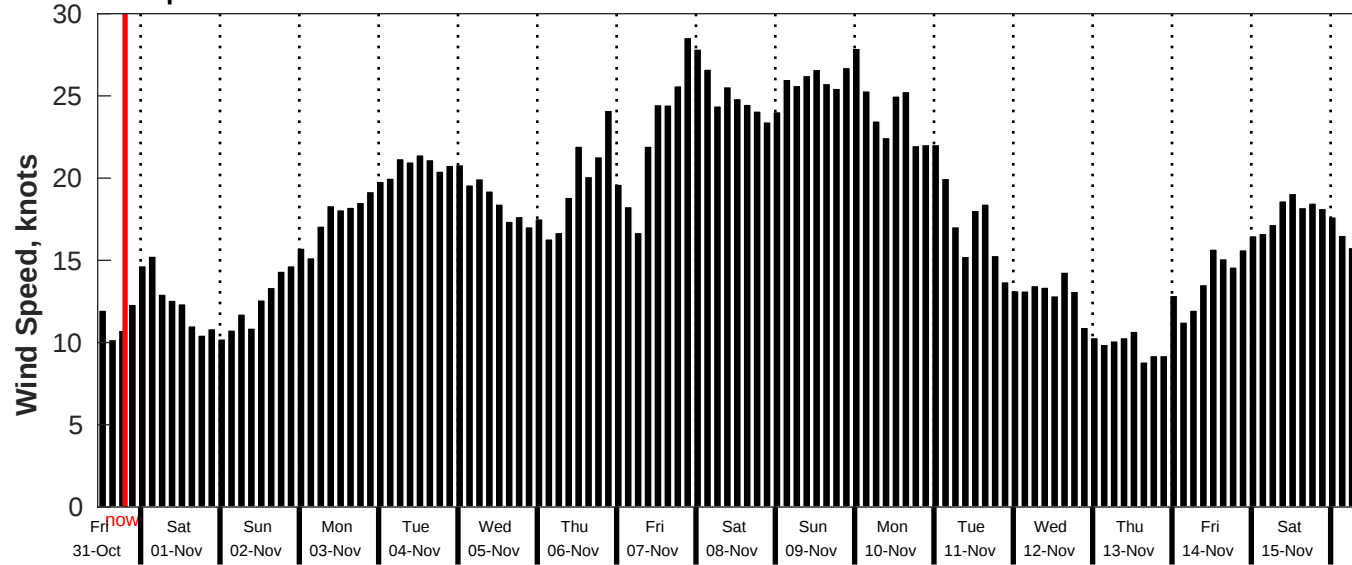
GFS Wind Speed Forecast for NDBC 52211 from 30-Oct-2025 11:00:00 to 15-Nov-2025 11:00:00
