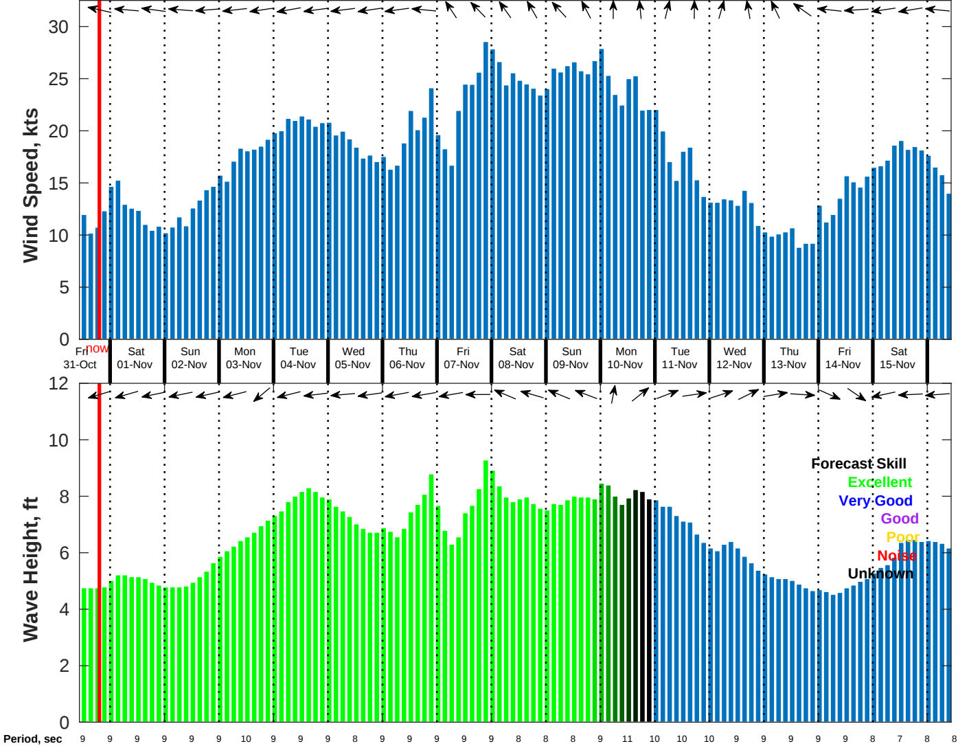
Wind & Wave Forecast for NDBC 52211 from 30-Oct-2025 11:00:00 to 15-Nov-2025 11:00:00
