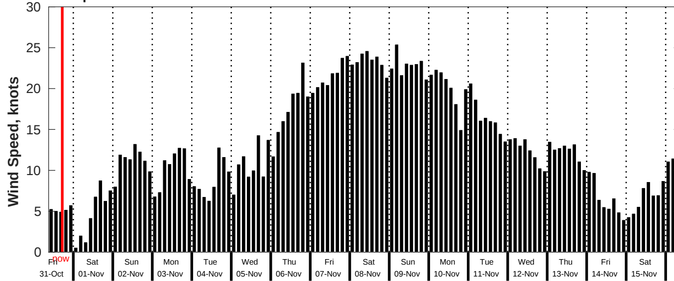
GFS Wind Speed Forecast for NDBC 52212 from 30-Oct-2025 09:00:00 to 15-Nov-2025 09:00:00
