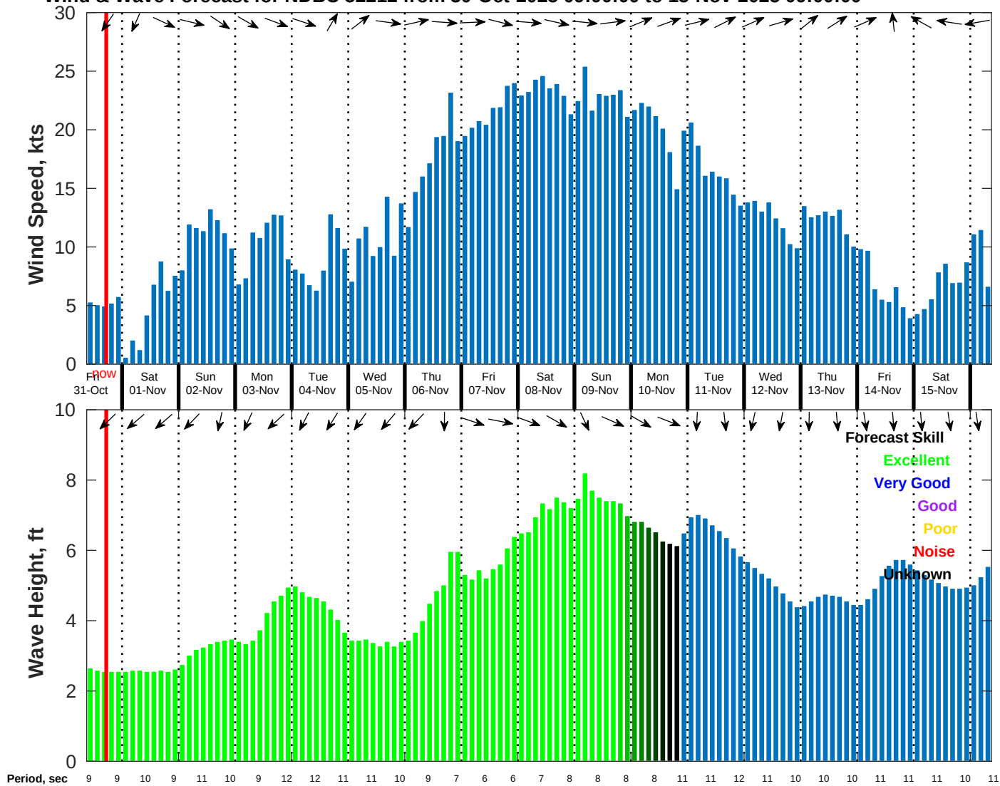
Wind & Wave Forecast for NDBC 52212 from 30-Oct-2025 09:00:00 to 15-Nov-2025 09:00:00
