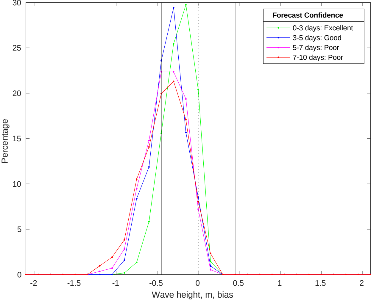
NDBC 52213 vs CMEMS Waves Bias Histogram: 30-Oct-2025
