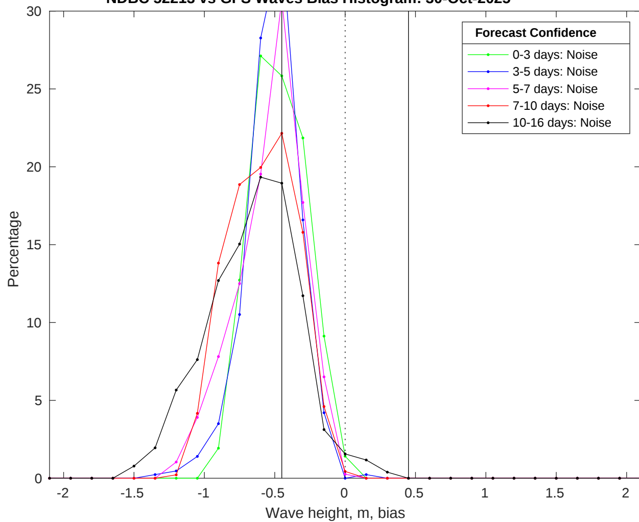
NDBC 52213 vs GFS Waves Bias Histogram: 30-Oct-2025
