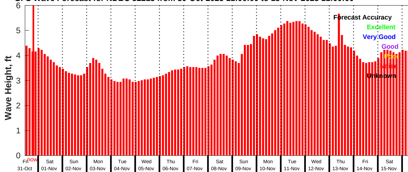
GFS Wave Forecast for NDBC 52213 from 30-Oct-2025 11:00:00 to 15-Nov-2025 11:00:00
