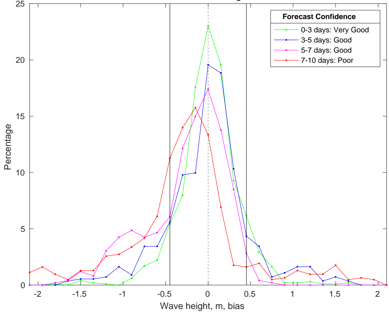
NDBC 41004 vs CMEMS Waves Bias Histogram: 31-Oct-2025
