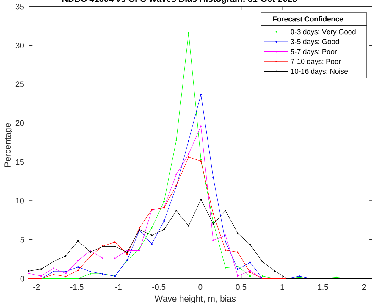
NDBC 41004 vs GFS Waves Bias Histogram: 31-Oct-2025
