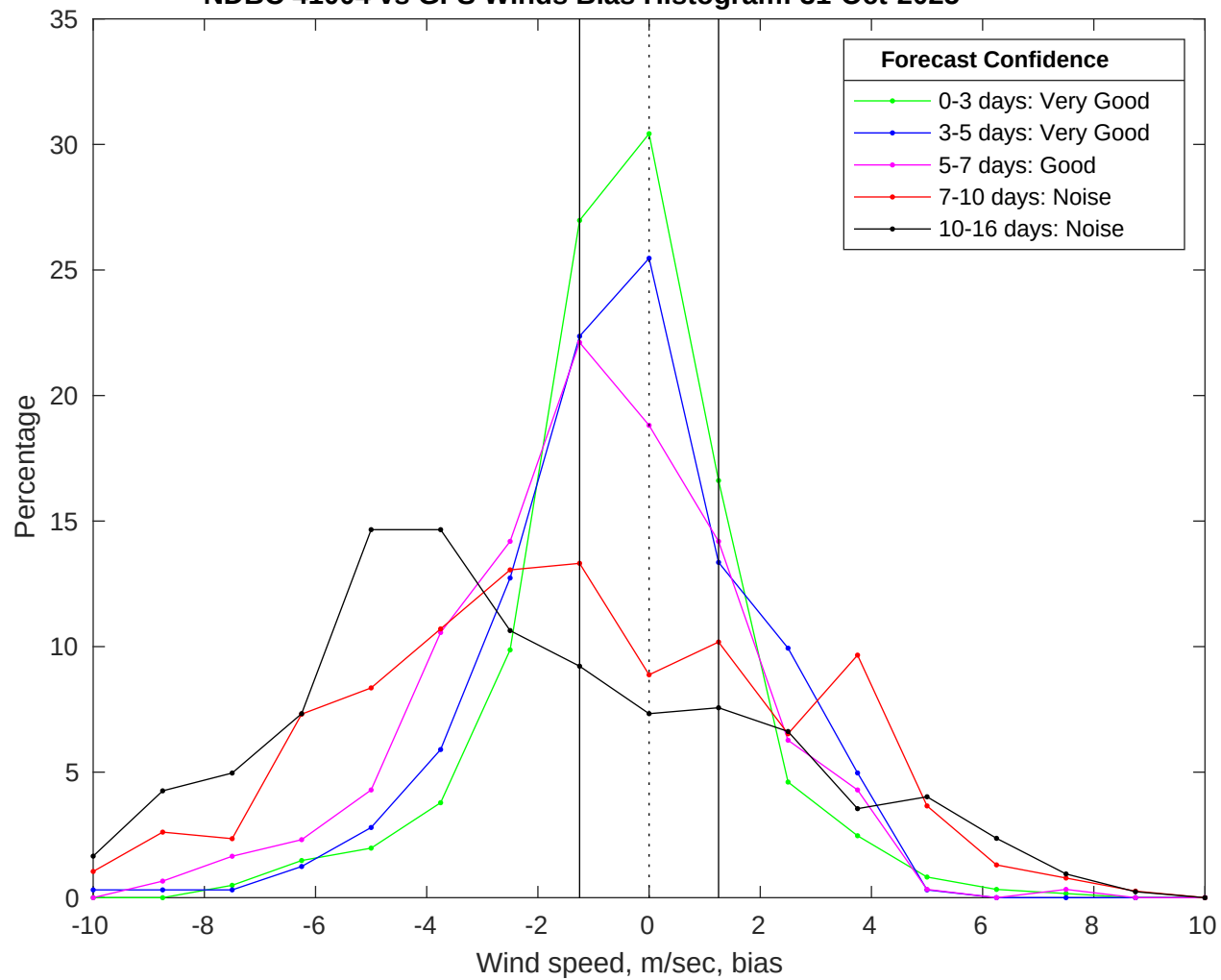
NDBC 41004 vs GFS Winds Bias Histogram: 31-Oct-2025
