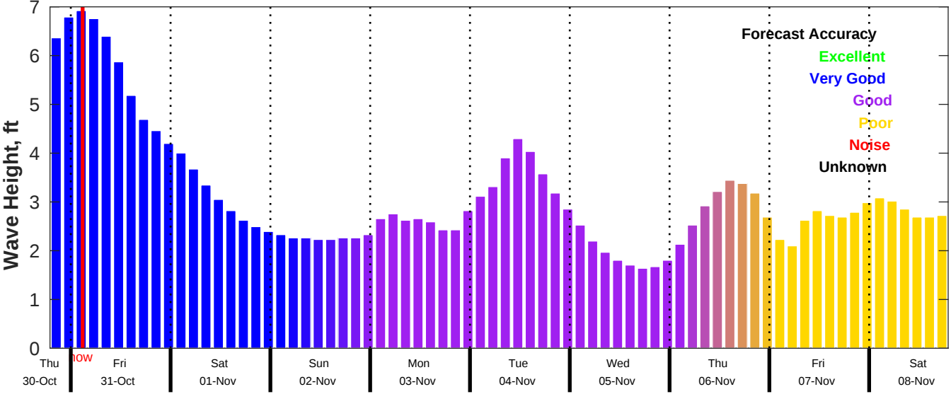
CMEMS Wave Forecast for NDBC 41004 from 30-Oct-2025 19:00:00 to 08-Nov-2025 19:00:00
