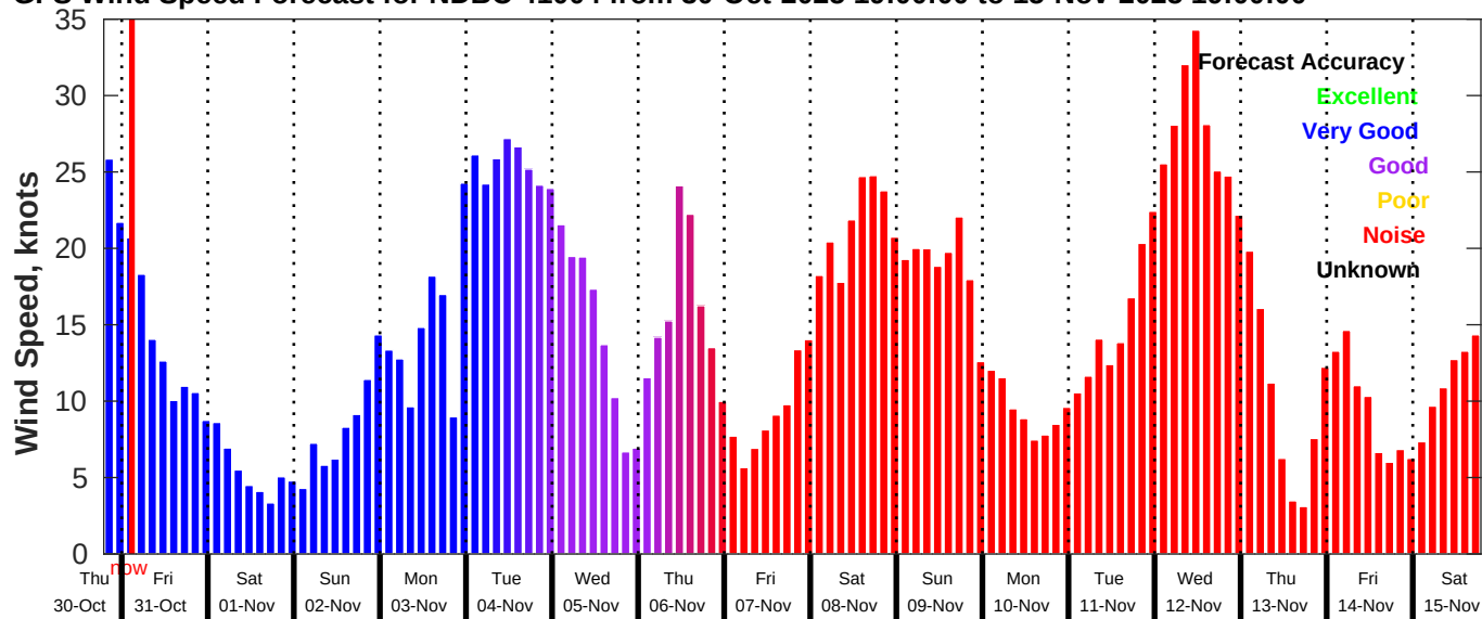
GFS Wind Speed Forecast for NDBC 41004 from 30-Oct-2025 19:00:00 to 15-Nov-2025 19:00:00
