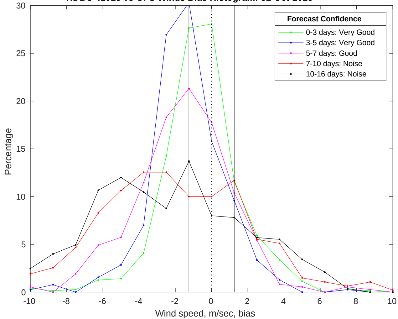
NDBC 41013 vs GFS Winds Bias Histogram: 31-Oct-2025
