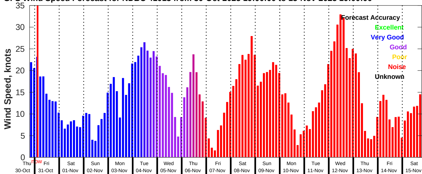
GFS Wind Speed Forecast for NDBC 41013 from 30-Oct-2025 19:00:00 to 15-Nov-2025 19:00:00
