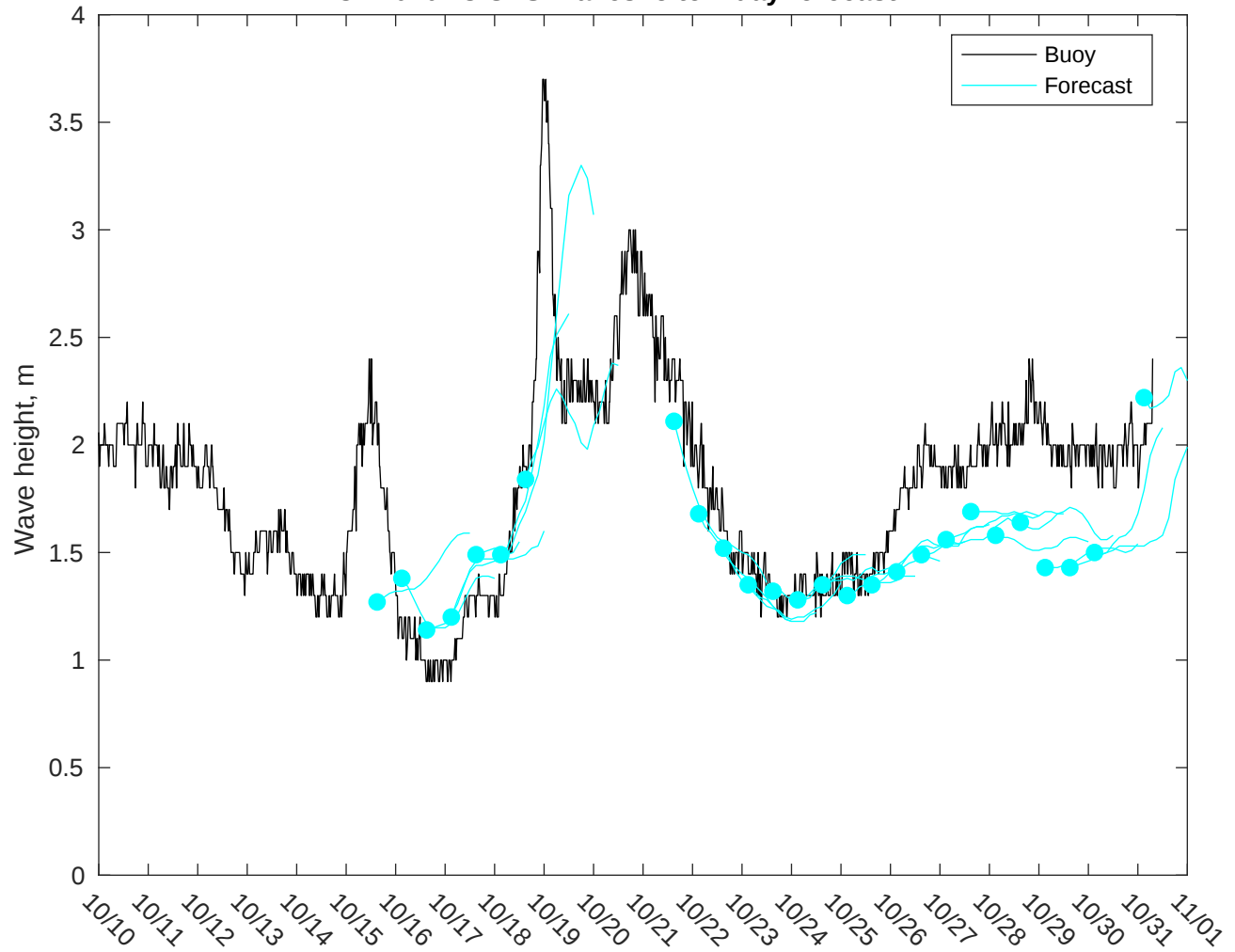
NDBC 41040 vs GFS Waves: 5 to 7 day forecast
