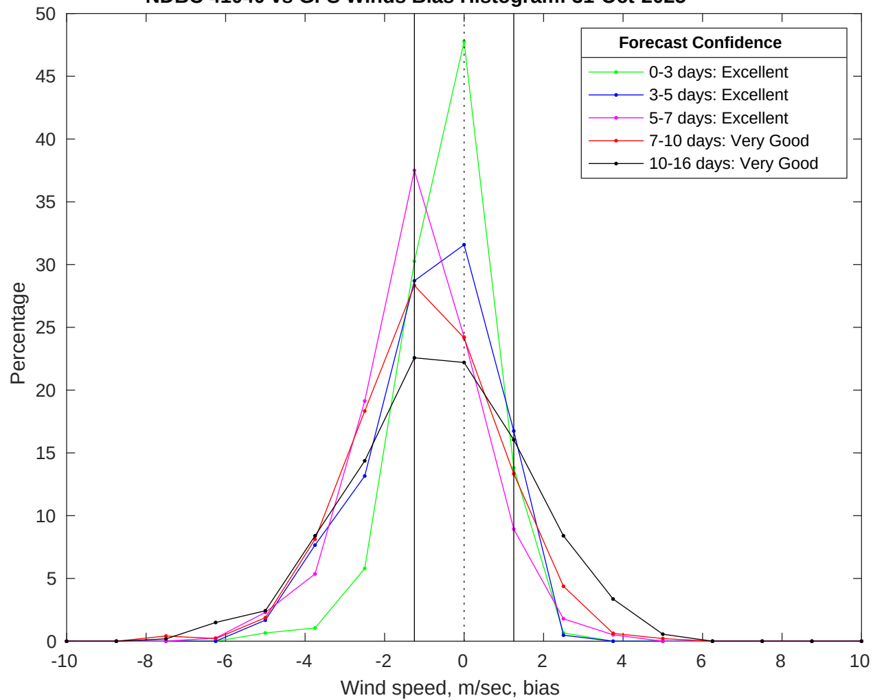
NDBC 41040 vs GFS Winds Bias Histogram: 31-Oct-2025
