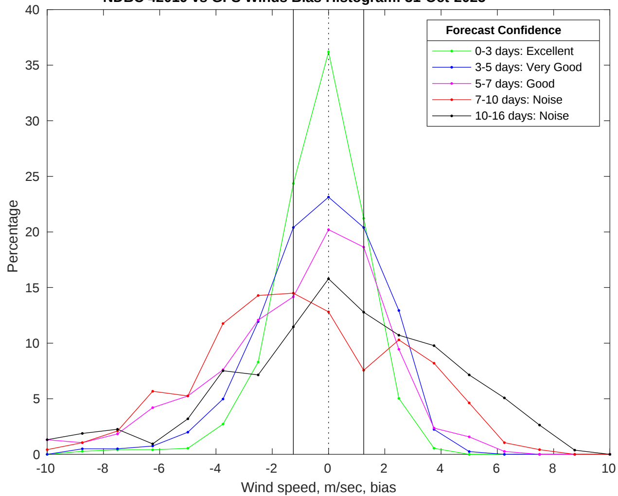
NDBC 42019 vs GFS Winds Bias Histogram: 31-Oct-2025
