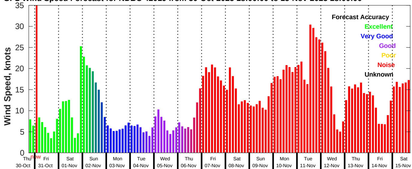
GFS Wind Speed Forecast for NDBC 42019 from 30-Oct-2025 18:00:00 to 15-Nov-2025 18:00:00
