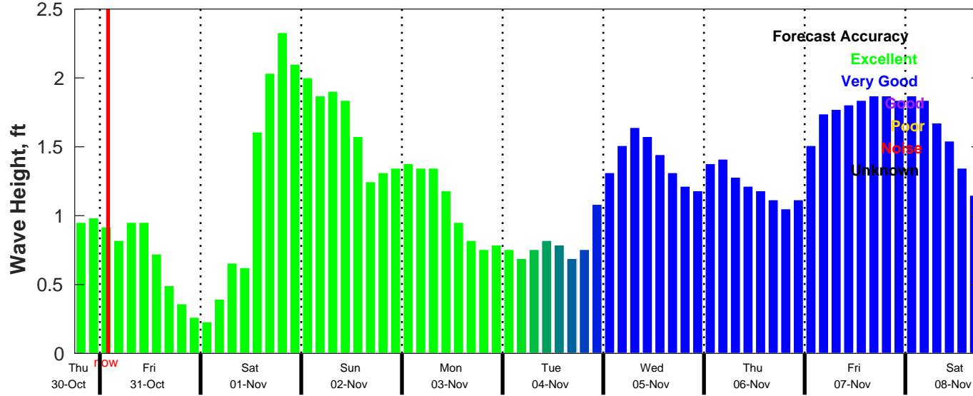
CMEMS Wave Forecast for NDBC 42035 from 30-Oct-2025 18:00:00 to 08-Nov-2025 18:00:00
